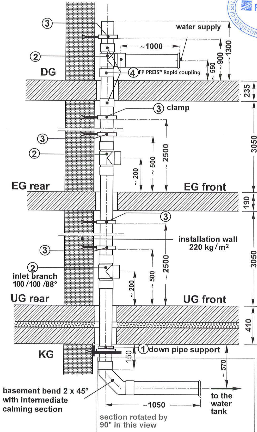
Figure 8 Installation plan of the Cast Iron Drainage System "FP PREIS® SML" mounted at the installation wall with different pipe clamps (drawing not to scale, dimensions in mm).
